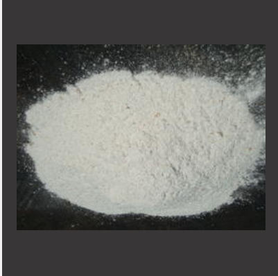
Silica Ramming Mass Premixed with Boron Oxide
